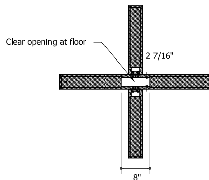
Horizontal section of typical base
