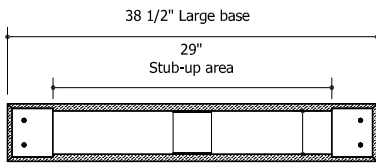
Horizontal section of Large base
