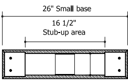
Horizontal section of Small Base
