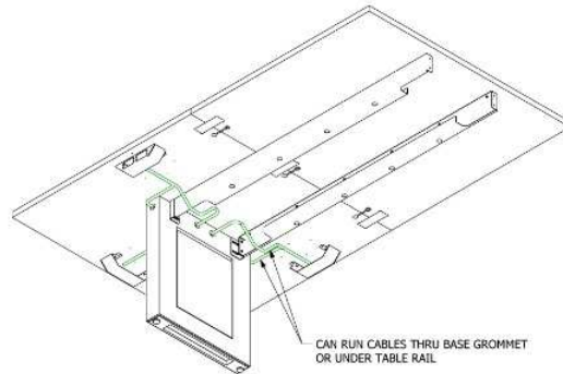
CABLING DIAGRAM: UNDER-MOUNT POWER OPTION
