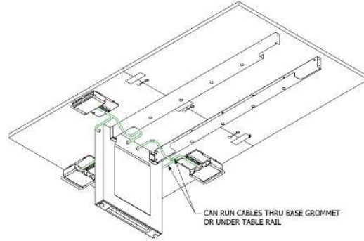
CABLING DIAGRAM: SLIDE-OUT POWER OPTION
