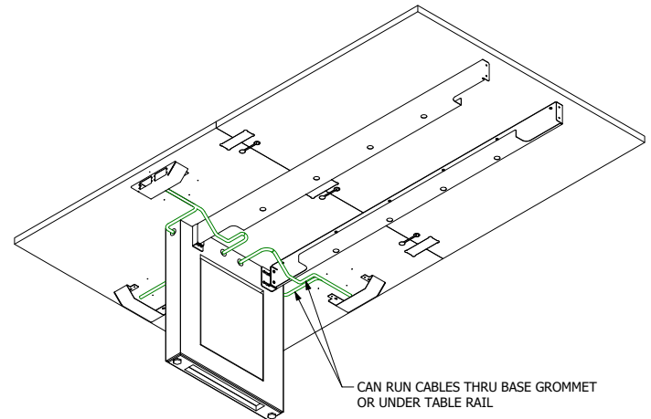
CABLING DIAGRAM: UNDER-MOUNT POWER OPTION
