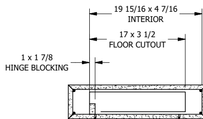
SECTION A-A INTERIOR CLEARANCES
